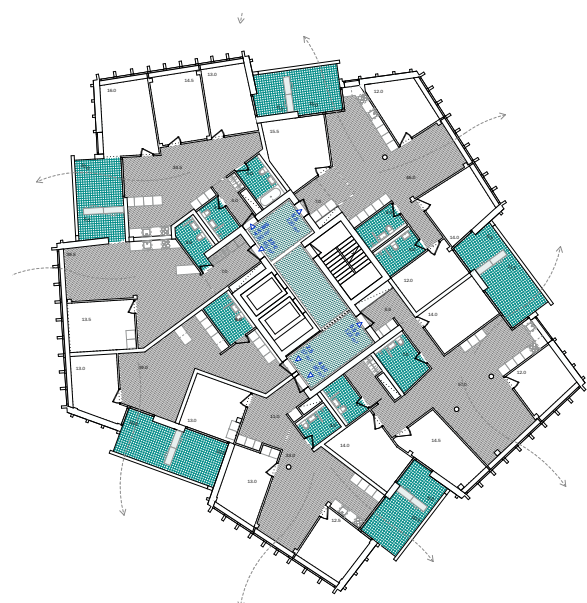
Grundriss PGW Baufeld B (2.+3. OG)
