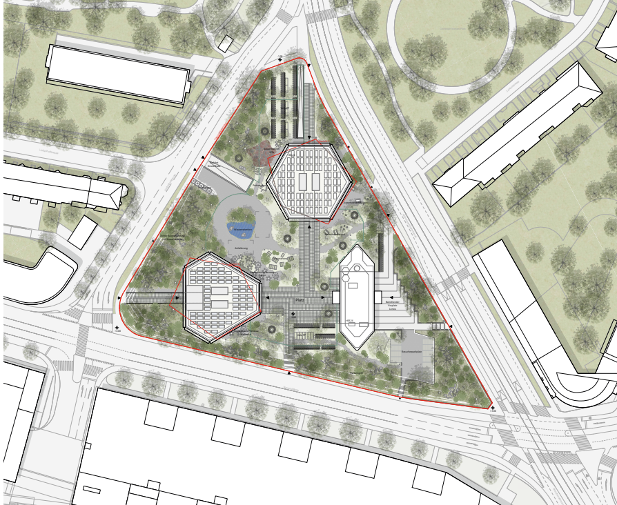
Situationsplan
